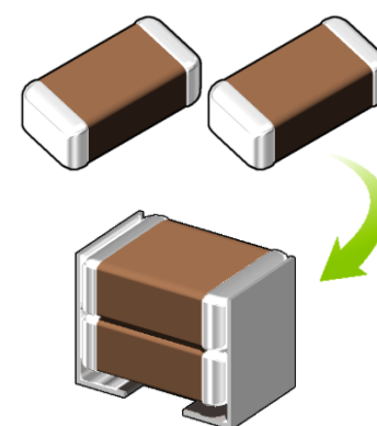
Double Cap Configuration
